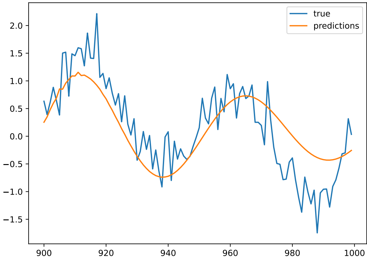
Final AR(16) forecast, m = 100
